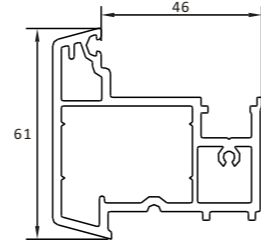
C403B FAKE MULLION
