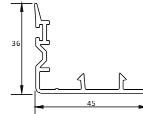
S404S 45MM INTERLOCKER
