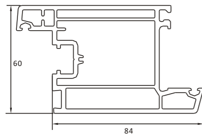
C406B DOOR SASH INTERNAL B
