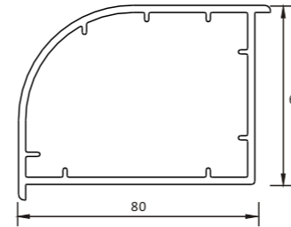
A407B CORNER CONNECTOR
