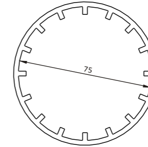
A402B BAY POST
