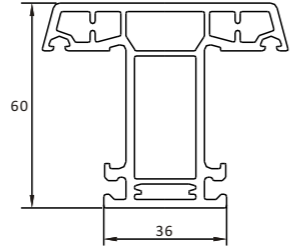
C403 FRAME MULLION/TRANSOM
