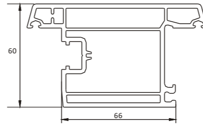
C405B DOOR SASH EXTERNAL B
