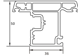
C404S WINDOW SASH B
