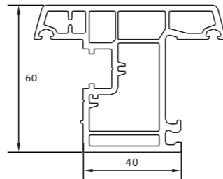
C404B WINDOW SASH B
