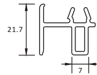
A411 SCREEN SASH ADAPTER
