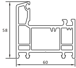
C401 MAIN FRAME
