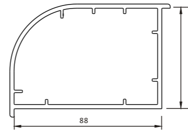
A407C CORNER CONNECTOR
