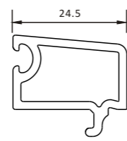
GB25.0 GLAZING BEAD
