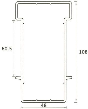
AP415 FRAME CONNECTOR
