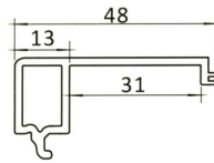
AP416 BEADS FOR BLINDS
