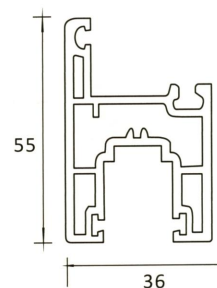
SP 409 36MM WINDOW SASH
