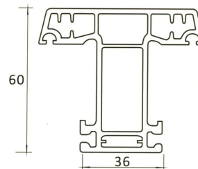
CP 403 FRAME MULLION/TRANSOM
