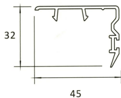
SP 404-S 42MM INTERLOCKER-SHORT
