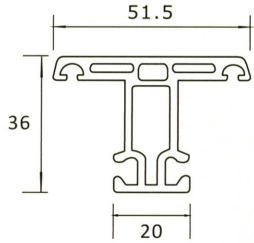
SP 410 36MM SASH MULLION
