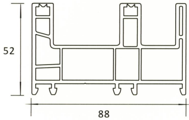
SP 413 88MM DOOR FRAME W/SCREEN
