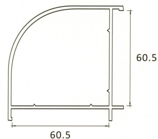
AP408 60-60MM CORNER CONNECTOR
