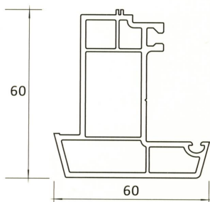
CP 403-B CASEMENT MULLION FOR DOUBLE SWING OPENING
