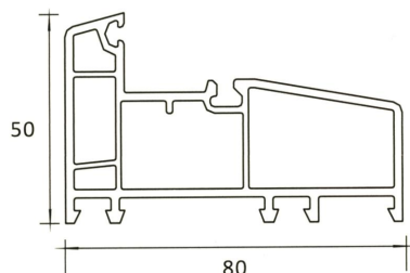
SP 408-B NARROW MULLION
