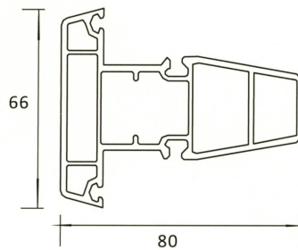
SP 415-B SASH/MULLION
