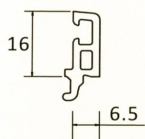
GB4-6.5 6.5MM GLAZING BEAD
