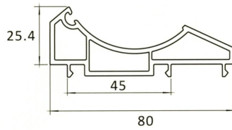
AP401-B BAY POST ADAPTOR 80
