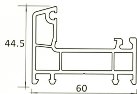
CP 402 SLIM WINDOW FRAME
