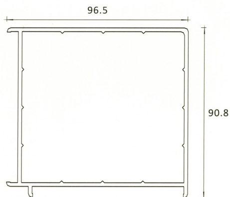
AP414 CURVED CORNER
