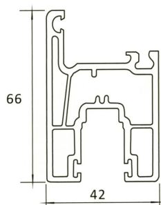
SP 402 42MM WINDOW SASH
