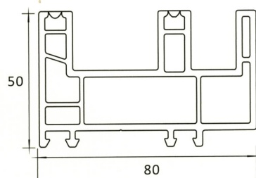
SP 406 80MM WINDOW FRAME W/SCREEN
