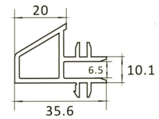
AP404-L 21MM FRAME CONNECTOR
