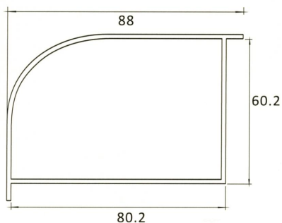
AP407 60-80MM CORNER CONNECTOR
