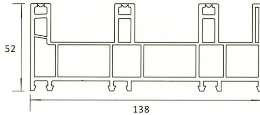
SP 413-B 138MM 3 TRACK DOOR FRAME W/SCREEN
