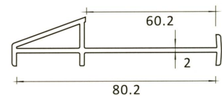
AP406-S 60-80MM FRAME CONNECTOR
