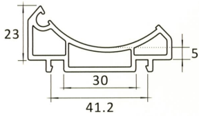
AP401 BAY POST CONNECTOR 60
