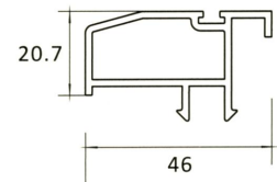
AP420 CLOSED FRAME FOR SWING DOOR
