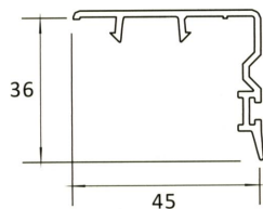
SP 404 42MM INTERLOCKER-ORIGINAL
