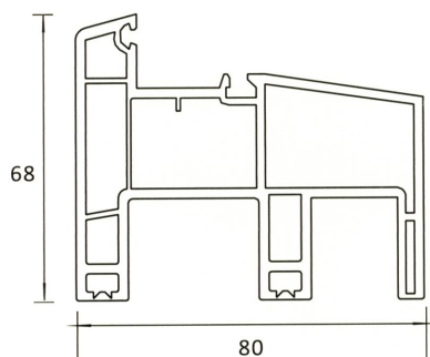
SP 407-C SLIM FRAME
