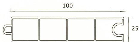
AP413 25MM TONGUE & GROOVE PANEL
