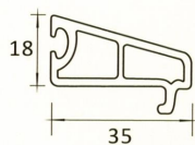
GB4-35 35MM GLAZING BEAD
