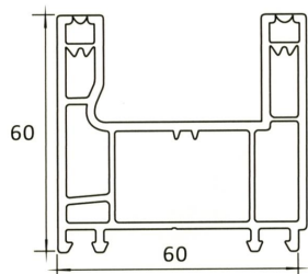
SP 401 60MM MAIN FRAME W/O SCREEN
