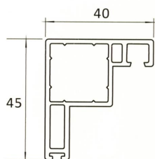
CP 407 INSECT SCREEN FRAME
