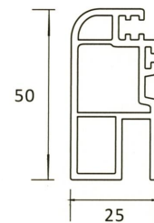
SP 416 INSECT SCREEN FRAME
