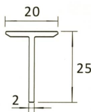
AP411 INSECT SCREEN INLINE ADAPTER
