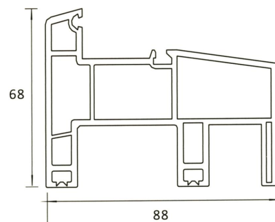
SP 407-B SLIM FRAME B
