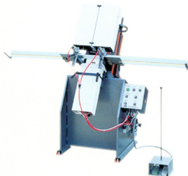
LXC01-3 AUTO WATER SLOT MILLING MACHINE(THREE AXIS)
